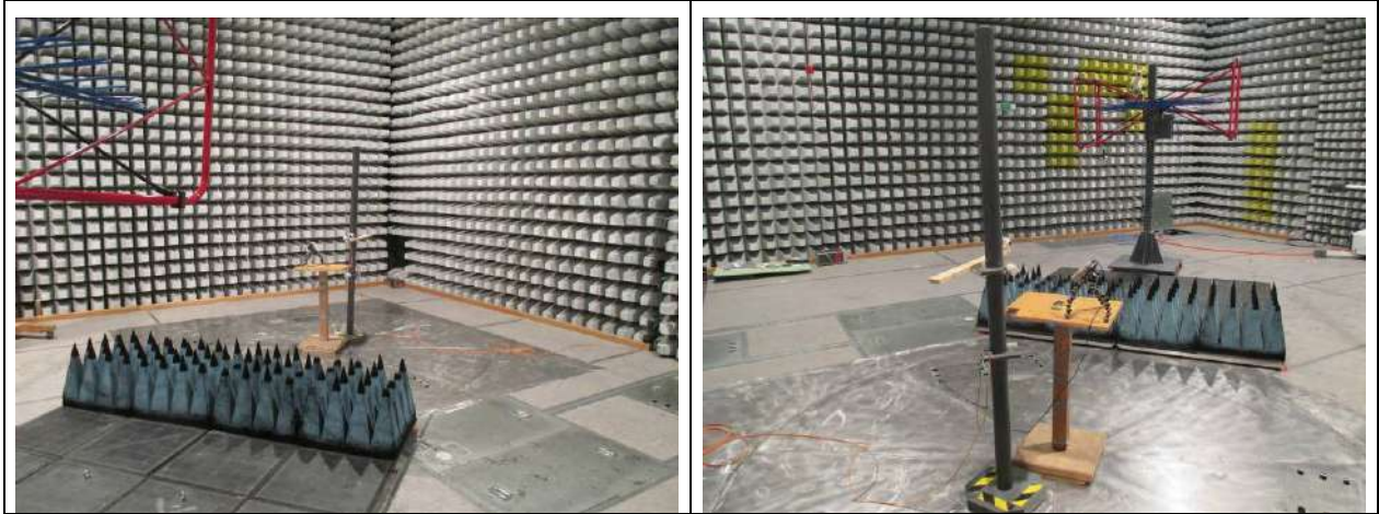
Figure 6-15: test setup for radio frequency electromagnetic fields 80 MHz to 1000 MHz
