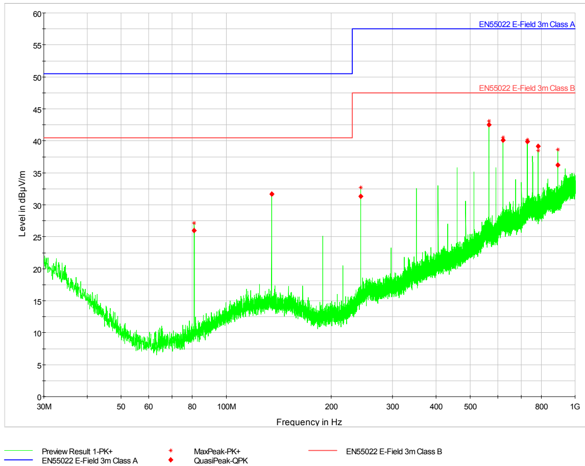
Figure 6-4: Graphical presentation Radiated disturbances 30 MHz to 1000 MHz
