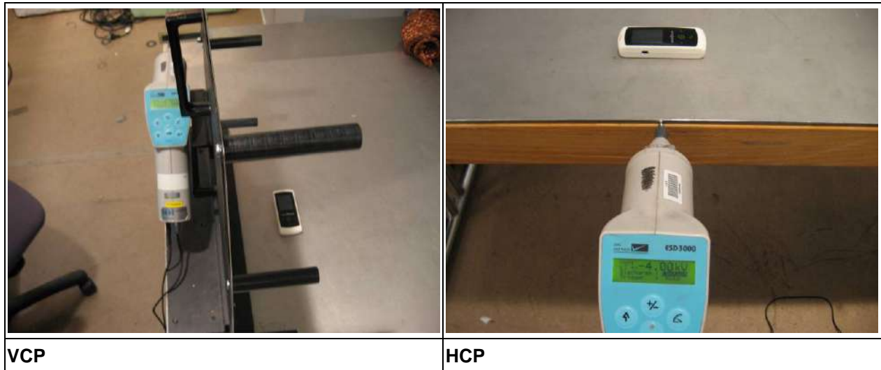
Figure 6-8: test setup for Electrostatic discharges
