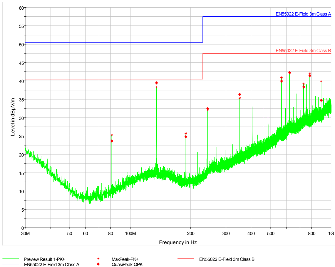
Figure 6-6: Graphical presentation Radiated disturbances 30 MHz to 1000 MHz
